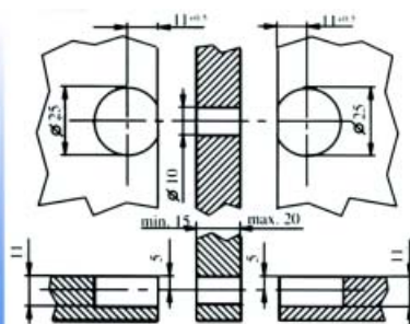
Kastverbinding type G98MA/G98FAI
